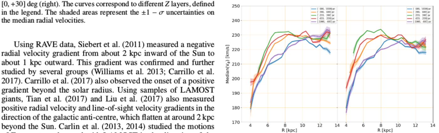
Fig. 13. Same as Fig. 12 for the median azimuthal velocity, \bar{V}_\phi .
