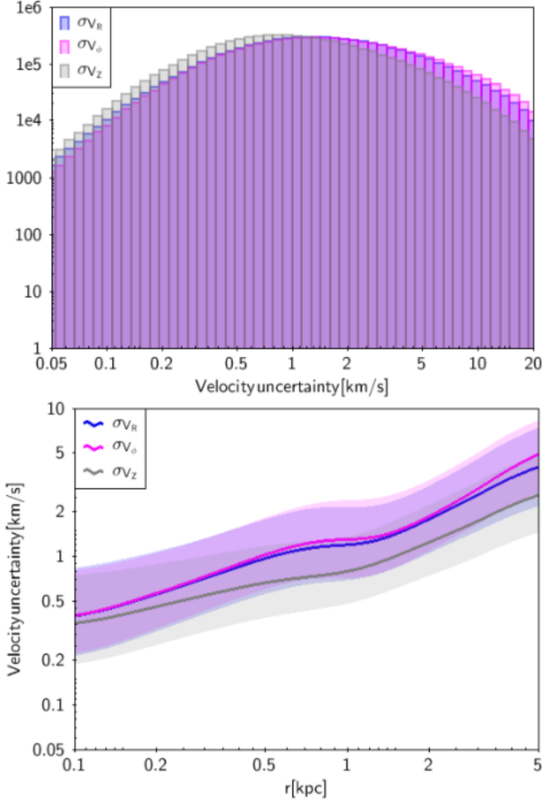
Fig. 4. Top : Histogram of velocity uncertainties in the Galactic cylindrical reference system ( V_R , V_\phi , V_z ) for the main sample. Bottom : Median uncertainties in velocity as a function of the heliocentric distance for the main sample. The 25% and 75% quartiles are shown as colour-shaded areas.
