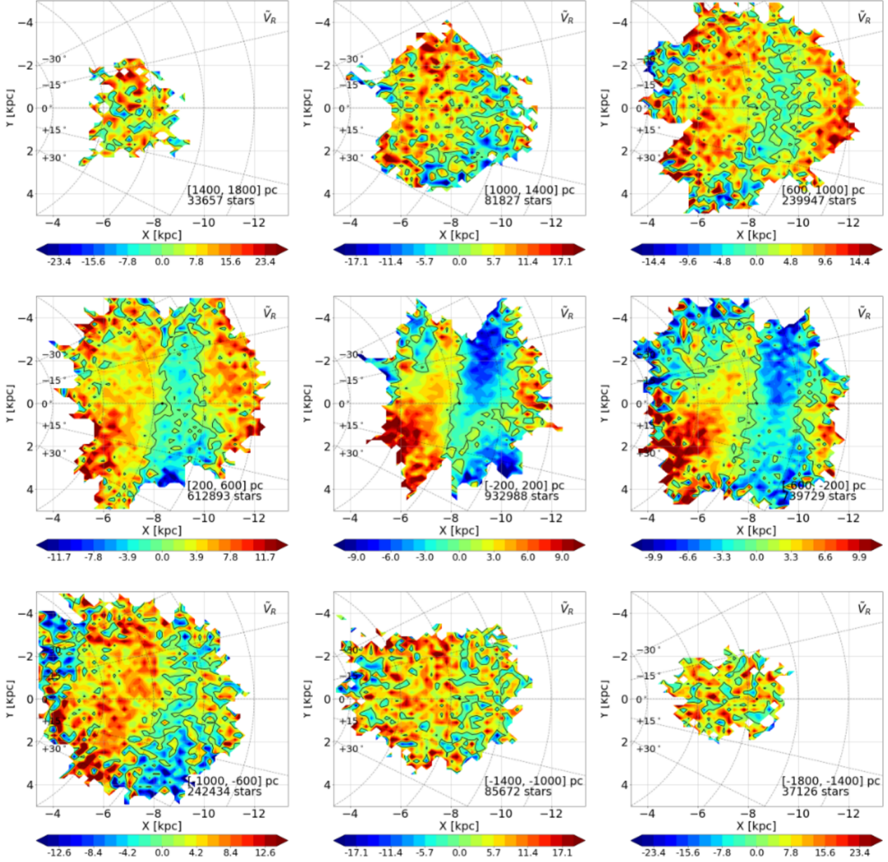
Fig. C.1. Mosaic of face-on maps of the median radial velocity, \bar{V}_R , of the giant sample. Each map corresponds to a Z layer of 400 pc height, from [+1400, +1800] pc (top left) to [−1800, −1400] pc (bottom right). In each map, the azimuths increase clockwise. They are labelled from −30 to +30 degrees on the left of the maps. The Sun is represented by a black dot at X = -8.34 kpc and Y = 0 kpc. The Galactic centre is located on the left side. The Milky Way rotates clockwise. The iso-velocity contours \bar{V}_R = 0 \text{ km s}^{-1} are pointed out as black lines. The numbers of stars used to produce the maps are given in the lower left corners.
