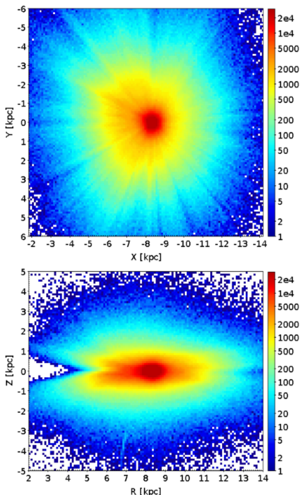
Fig. 2. Top : Surface density in the (X, Y) plane for the stars in the main sample that have available extinction-corrected photometry (number of stars per bin of 100\text{pc} \times 100\text{pc} ). Bottom : Same for the (R, Z) plane.
