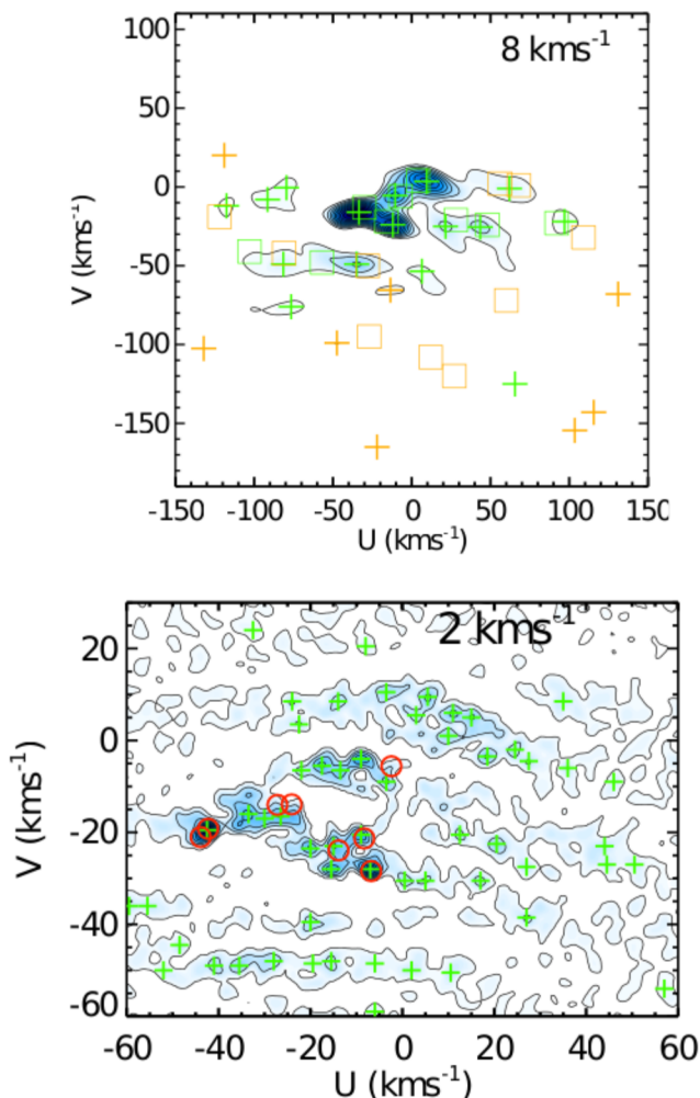
Fig. 23. Wavelet transform coefficients of the velocity plane in the solar neighbourhood showing the substructures at different scales. Top : Scales of around 8 \text{ km s}^{-1} . The green and orange symbols mark peaks that are > 3\sigma and 2 - 3\sigma significant, respectively, for DR2 (crosses) or for the RAVE sample (squares) from the study of Antoja et al. (2012) (their table 2). Bottom : Scales of around 2 \text{ km s}^{-1} . The green crosses mark peaks that are > 3\sigma significant. The red circles mark peaks for the velocity positions of nearby open clusters that are located at distances closer than 200 pc (see text). This panel shows a zoom-in on the central parts of the velocity plane.
