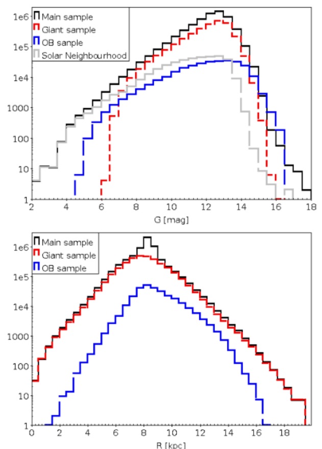
Fig. 3. Top : Histogram of the G apparent magnitude for the four working samples. Bottom : Histogram of the Galactic radius for the main, giant, and OB samples. Stars in the solar neighbourhood sample are located at d < 200 \text{ pc} (see Sect. 2).
