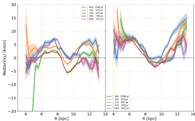
Fig. 12. Median radial velocities, \bar{V}_R , of the giant sample as a function of Galactic radius for two azimuth slices: [-30, 0] degrees (left), and [0, +30] deg (right). The curves correspond to different Z layers, defined in the legend. The shaded areas represent the \pm 1 - \sigma uncertainties on the median radial velocities.
