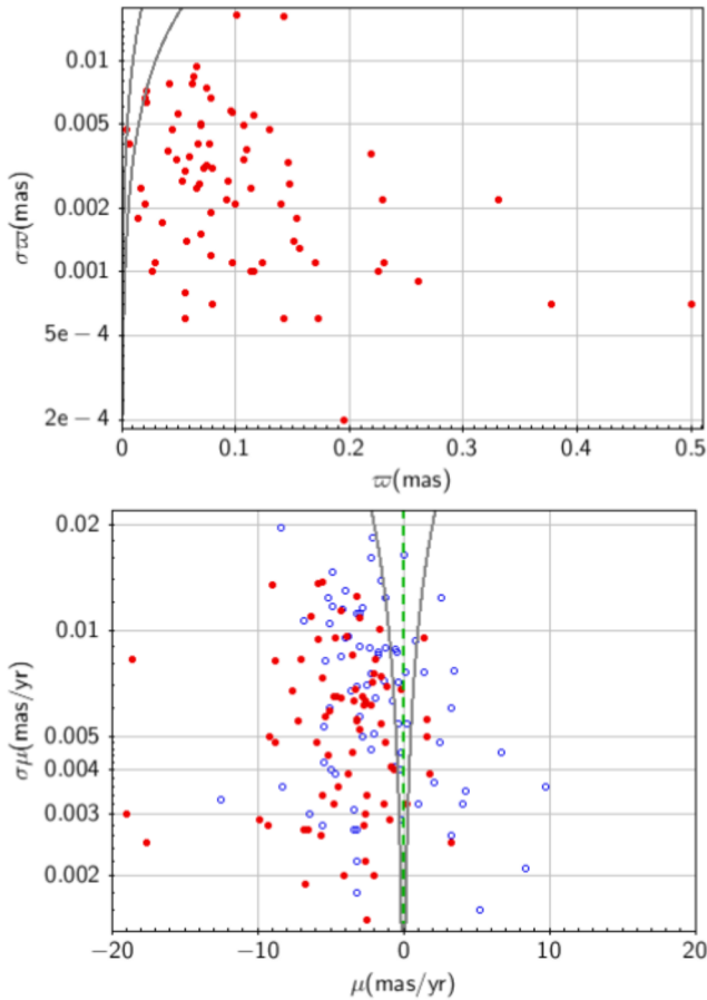
Fig. 7. Top : Parallax error against the Gaia parallax as determined from the Gaia data for 75 globular clusters. The black curves are the 1 and 3 \sigma limits. The vertical dashed line corresponds to 3 times our estimate of the systematic error on the parallax. Bottom : PM errors against the PMs in right ascension (open circles) and declination (solid circles) for the clusters in our sample. The curves represent the value of the PM for 100 \sigma_\mu . The PM measurement has a significance lower than 10 \sigma only for NGC 6453, for which \mu_{\alpha^*}/\sigma_{\mu_{\alpha^*}} \sim 4 .
