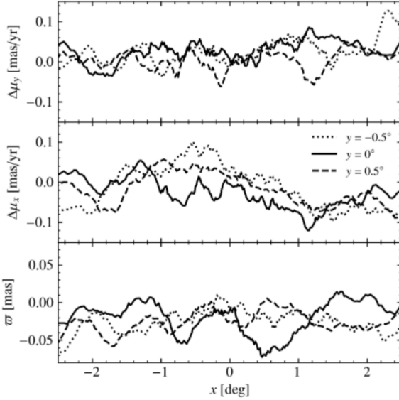
Fig. A.10. Parallaxes and residual PMs of sources in the LMC. The lines show the median value as a function of coordinate position x for all LMC sources within 0.2^\circ stripes centred at y = -0.5, 0 or 0.5^\circ . Residual PMs are calculated after subtraction of a model disc with parameters determined using only sources within 3^\circ of the centre. The non-zero values are due to both the systematic errors in the Gaia data and the differences between the simple disc model and the true dynamics of the LMC.
