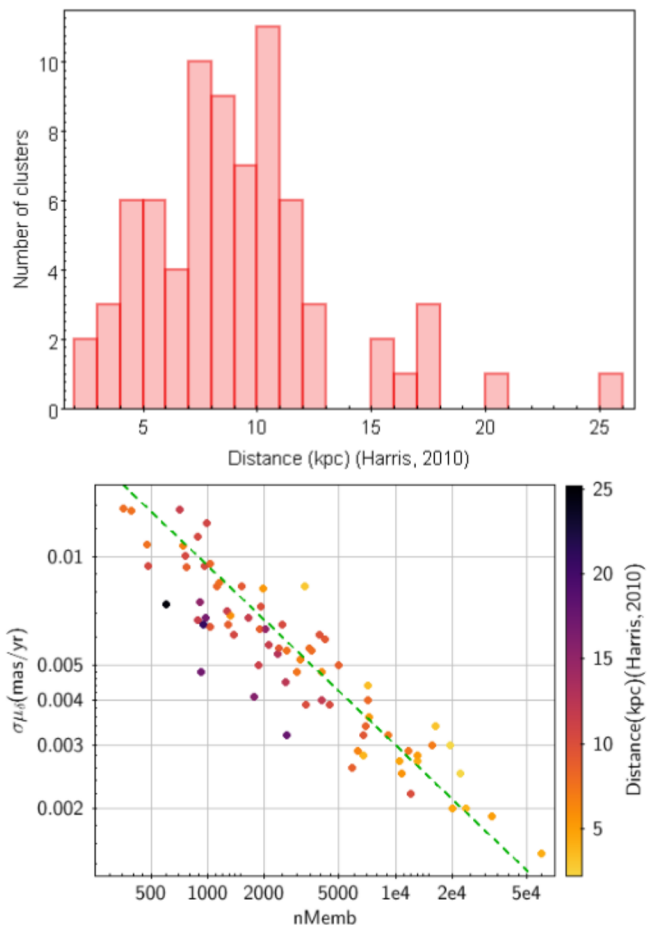
Fig. 1. Top : Distance distribution of the 75 globular clusters included in the present study. Bottom : Standard uncertainties on the PM in declination as a function of number of cluster members nMemb used in the solution. The diagonal line represents a fit to the relation \sigma_{\mu_\delta} = a/\sqrt{nMemb} where we find a = 0.3 [mas/yr]. A similar dependence on the number of members is found for the parallax uncertainty (with a = 0.15 [mas]) and for \sigma_{\mu_\alpha} (where a = 0.25 [mas/yr]).
