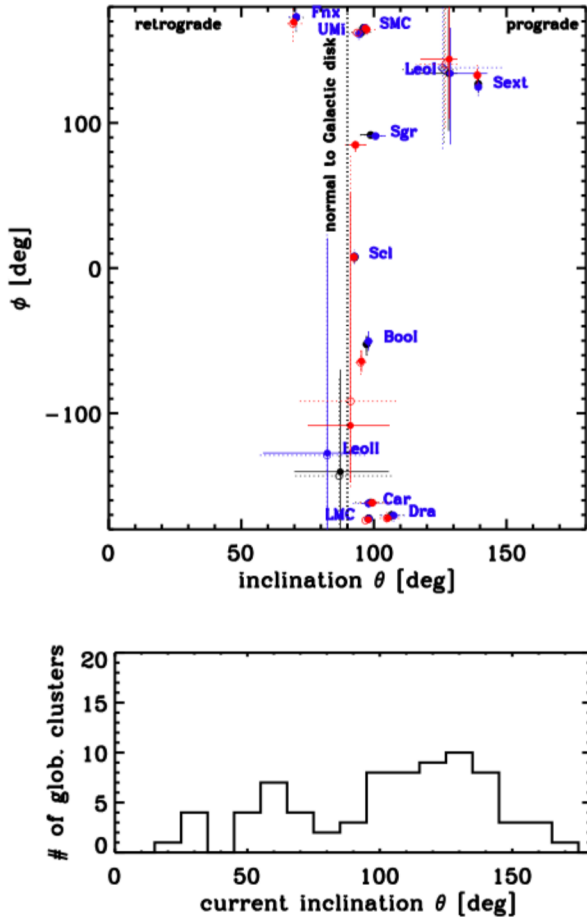
Fig. 23. Top : Orientation of the time-averaged orbital plane, defined by the angular momentum angles ( \phi, \theta ) for the different dwarfs for the various potentials. The colours and error bars are the same as in Fig. 22, and open and solid circles are the median values obtained by including or excluding our estimate of the systematic error on the PMs. Most dwarfs have highly inclined orbits with respect to the Galactic plane (i.e. \theta \sim 90^\circ ). Their variation in orientation (angle \phi ) over the 10 Gyr of integration is much smaller than the size of the error bars. Bottom : Histogram showing the present-day inclination of the orbits for the globular clusters.
