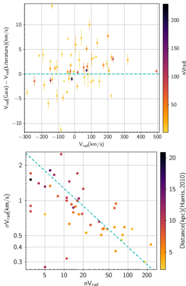
Fig. 9. Top : Comparison between the ground-based and Gaia radial velocities for 52 clusters with at least two measurements. Bottom : Standard uncertainties on the mean radial velocities as a function of the number of stars contributing to the mean. The diagonal line shows the effect of an additional contribution of 4 \text{ km s}^{-1} originating from the internal velocity dispersion.
