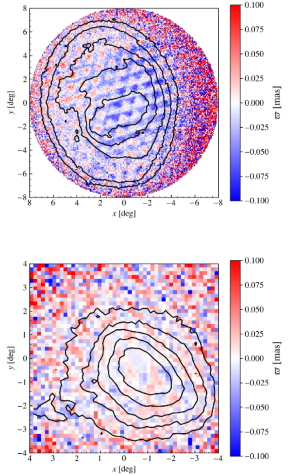
Fig. A.9. Measured parallaxes of stars in the LMC (upper panel) and SMC (lower panel). The banding associated with the Gaia scanning law is clearly visible.
