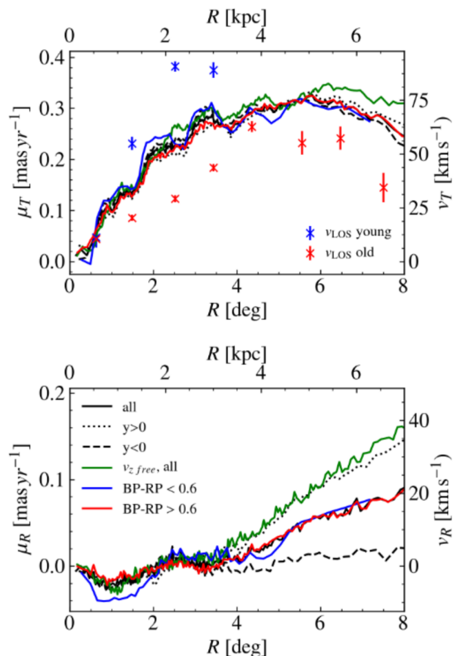
Fig. 18. Rotation curve (top) and median v_R (bottom) of the LMC. The assumed values for the centre-of-mass velocity and orientation of the disc ( i and \Omega ) are taken from a fit to all stars within angular radii \rho < 3^\circ of the LMC centre. Angular distances and velocities given on the lower and left axes have been converted to real-space values on the upper and right axes assuming a distance to the LMC of 50.1 kpc (Freedman et al. 2001). The points shown in the upper panel are derived from observed line-of-sight velocities of old and young stars by van der Marel & Kallivayalil (2014, their Table 4.)
