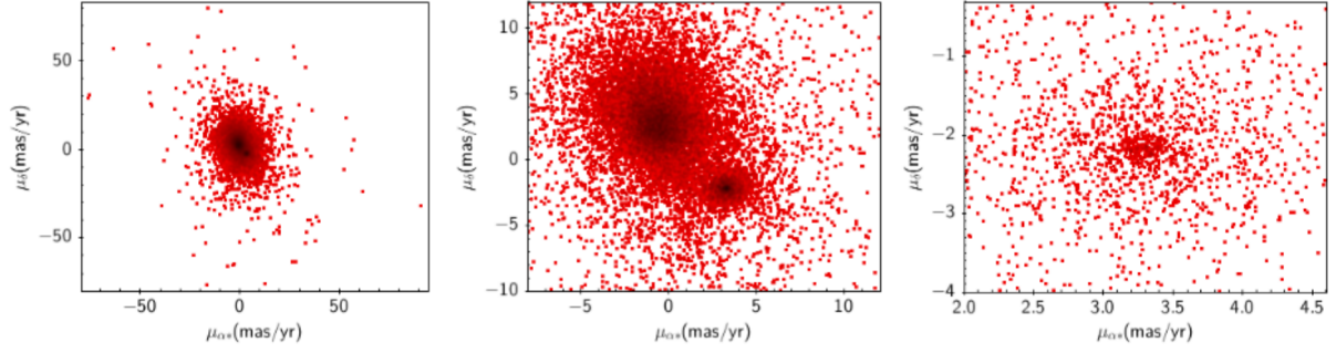
Fig. A.1. PM of stars within 0.5 deg. from the centre of NGC2298 as extracted from the GACS archive. Left : All \sim 259000 stars. Middle : Zoom-in on the PM field, which shows a concentration of the stars near position (3.2, -2.2) mas yr ^{-1} corresponding to cluster members. Right : Another zoom-in on the PM field for the cluster.
