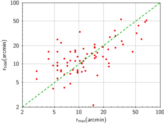
Fig. 4. Comparison between the tidal radii r_t (according to Harris10) of the 75 globular clusters in our sample and the maximum radii at which we have been able to detect cluster members in the present study. The diagonal line represents the one-to-one relation.
