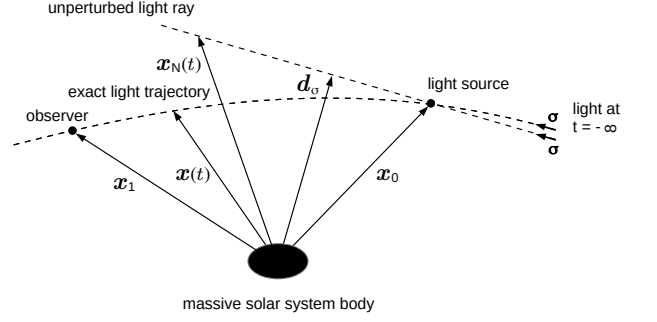
Figure 1: A geometrical representation of the propagation of a light signal through the gravitational field of a massive solar system body at rest. The light signal is emitted by the light source at \mathbf{x}_0 and propagates along the exact light trajectory \mathbf{x}(t) . The three-vector \mathbf{x}_1 points from the origin of the coordinate system towards the spatial position of the observer. The unit tangent vector along the light trajectory at past infinity is \boldsymbol{\sigma} . The unperturbed light ray \mathbf{x}_N(t) is given by Eq. (12) and propagates in the direction of \boldsymbol{\sigma} along a straight line through the position of the light source at \mathbf{x}_0 . The impact vector \mathbf{d}_\sigma of the unperturbed light ray is given by Eq. (21).
