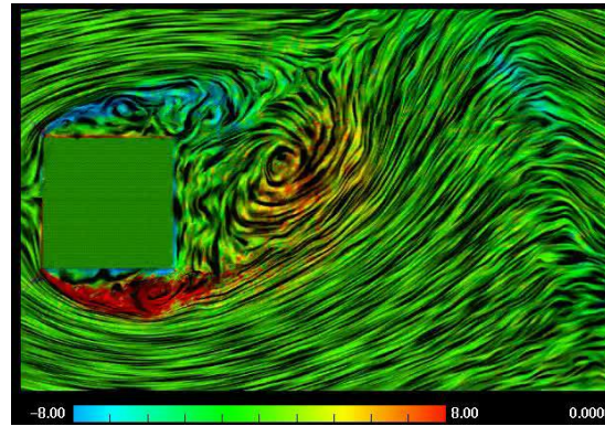
Re = 22000
