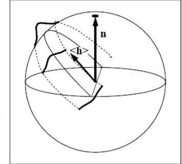
Figure 12: Microgeometry of velvet (left) and p(\mathbf{h}) used to model it (right).
