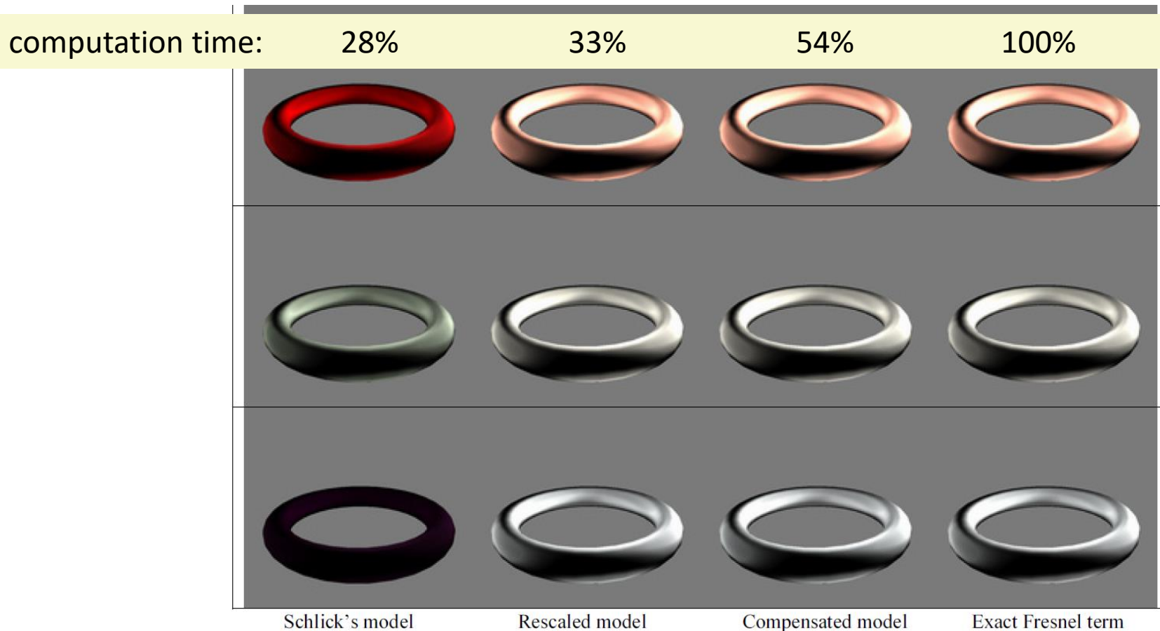
Figure 7. Copper, silver and aluminum rings rendered with different Fresnel approximations.
